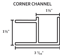
Product Item Product Name QWC001 Corner Channel -use for outside/inside corner applications.
